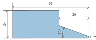
SCHARFSCHIENE 66/24 20°
